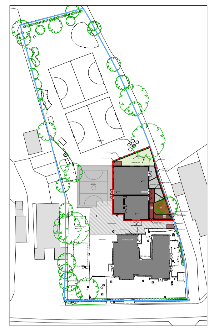
Location plan 1:1000
