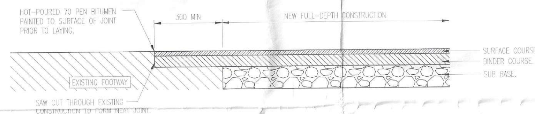
TYPICAL TIE-IN DETAIL TO EXISTING FOOTWAY CONSTRUCTION SCALE 1:10
