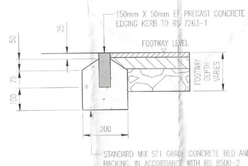
EDGING KERB (EF) DETAIL SCALE 1:10
