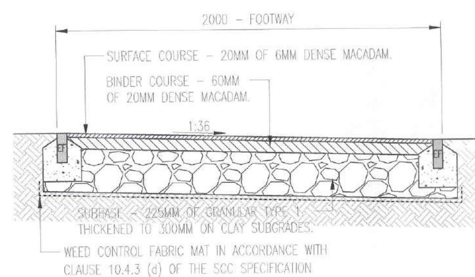
SECTION THROUGH INDEPENDENT FOOTWAY SCALE 1:20
