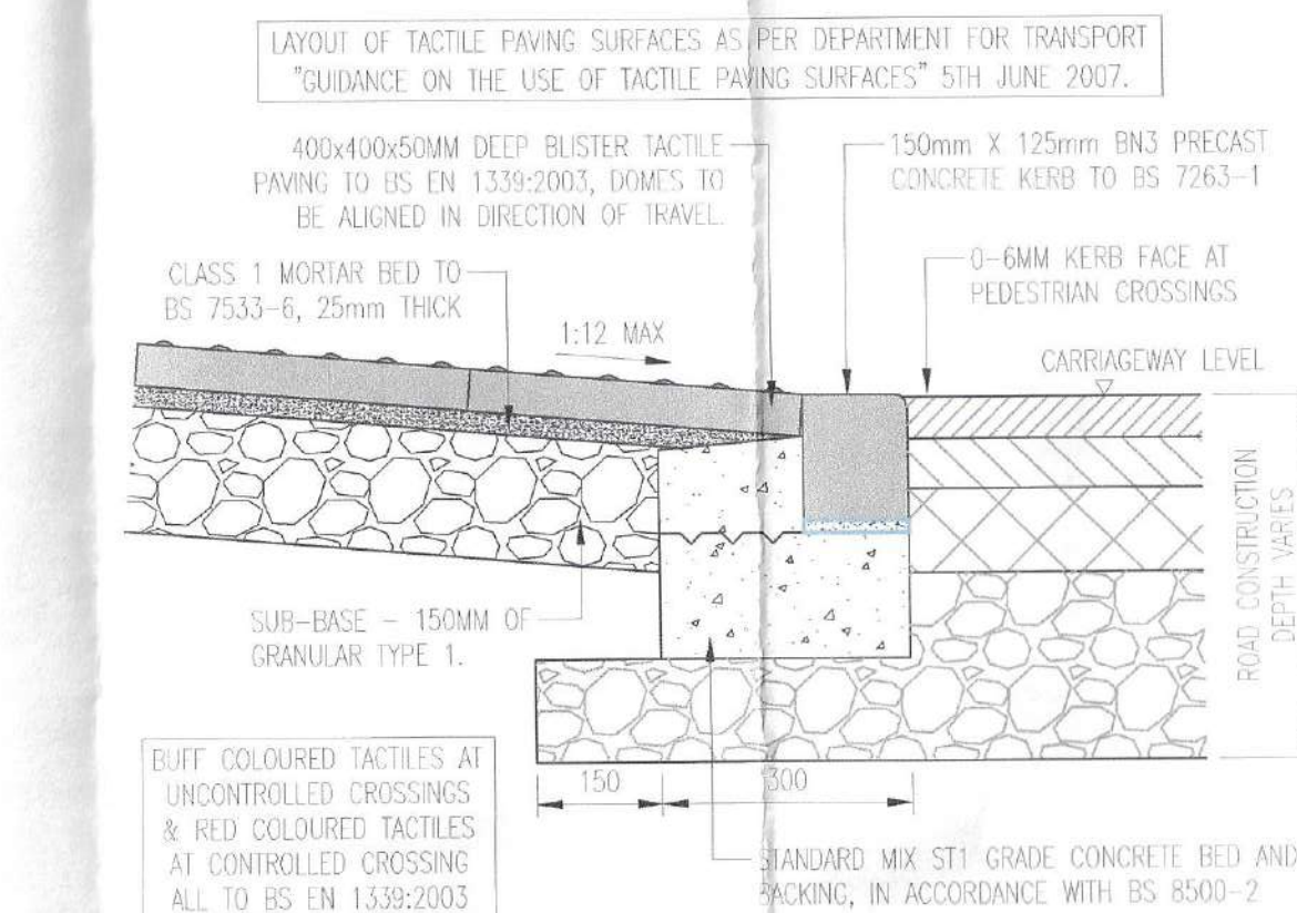
TYPICAL SECTION THROUGH PEDESTRIAN CROSSING SCALE 1:20
