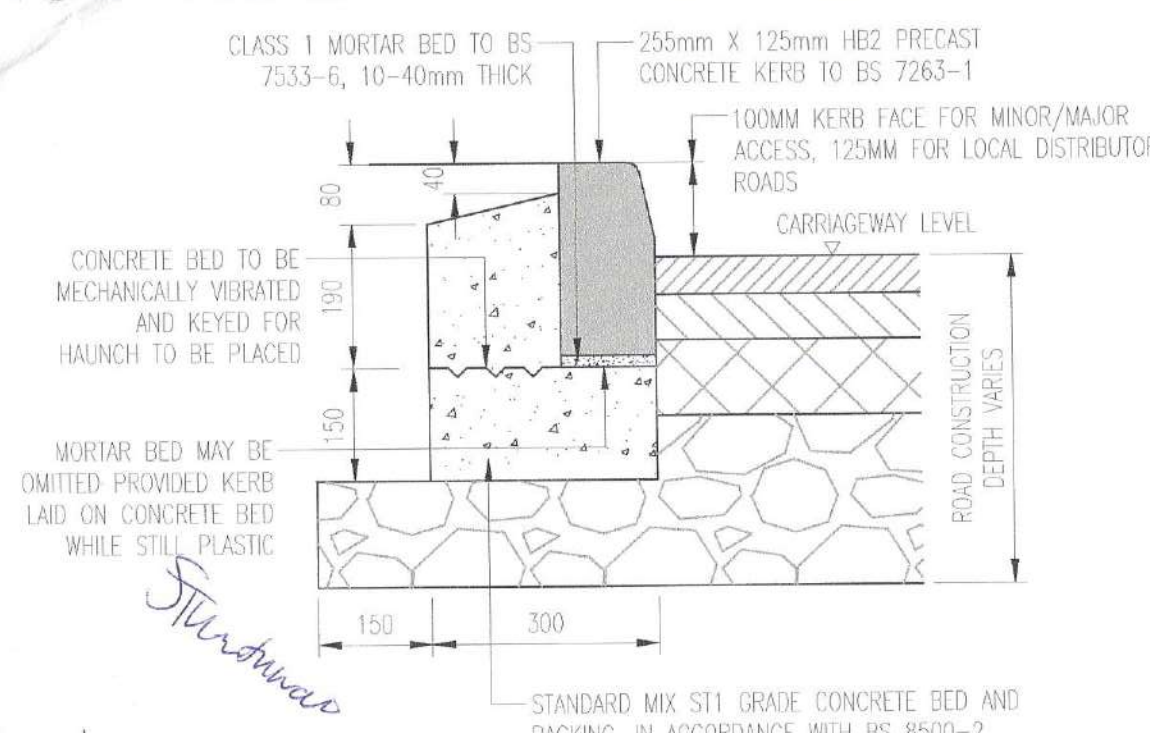
HALF-BATTERED KERB (HB2) DETAIL SCALE 1:10
