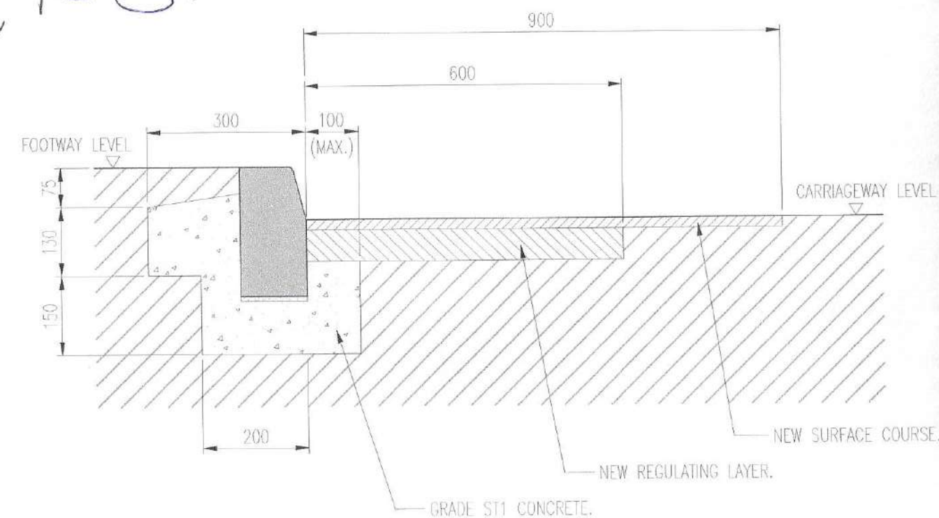
HALF-BATTERED KERB (HB2) DETAIL SCALE 1:10
