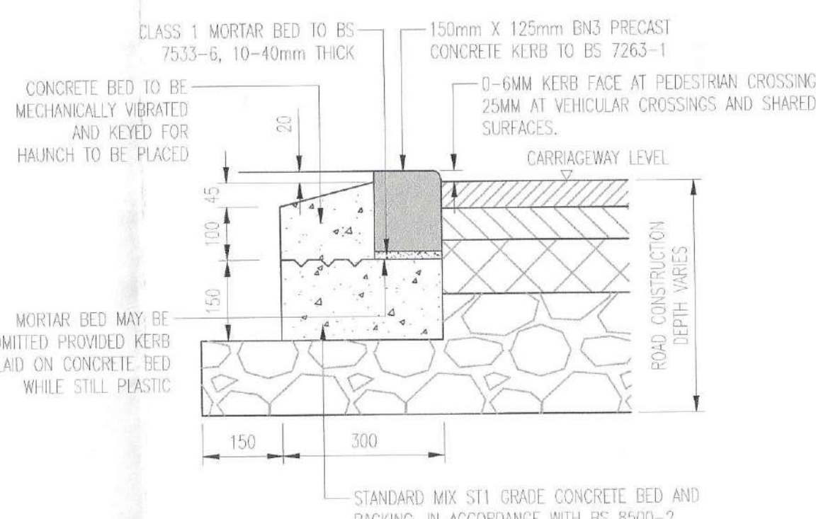
BULL-NOSE KERB (BN3) DETAIL SCALE 1:10
