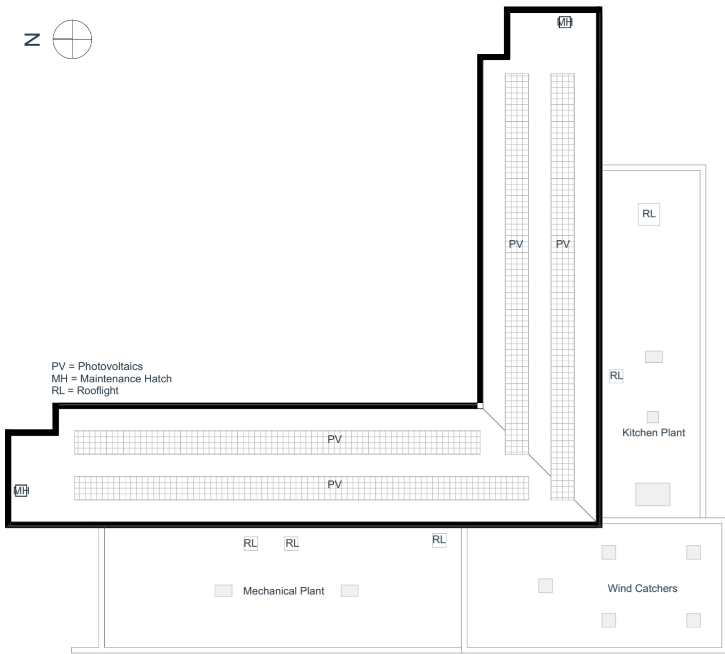
Roof Plan | NTS
