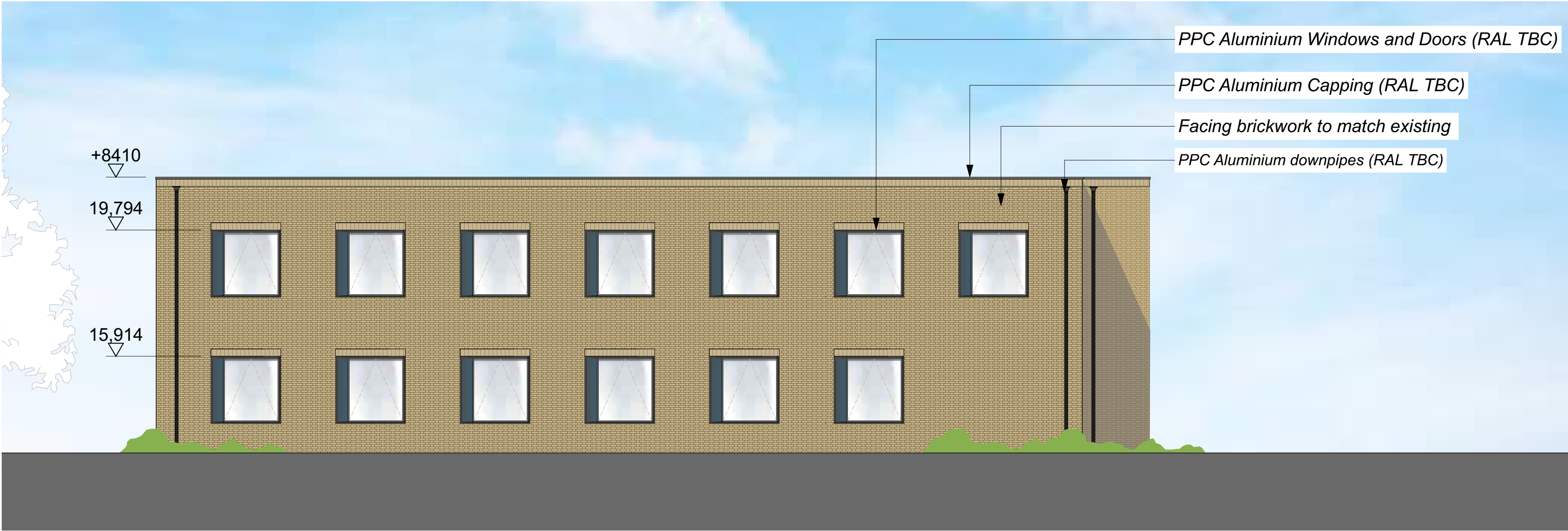
North Elevation
