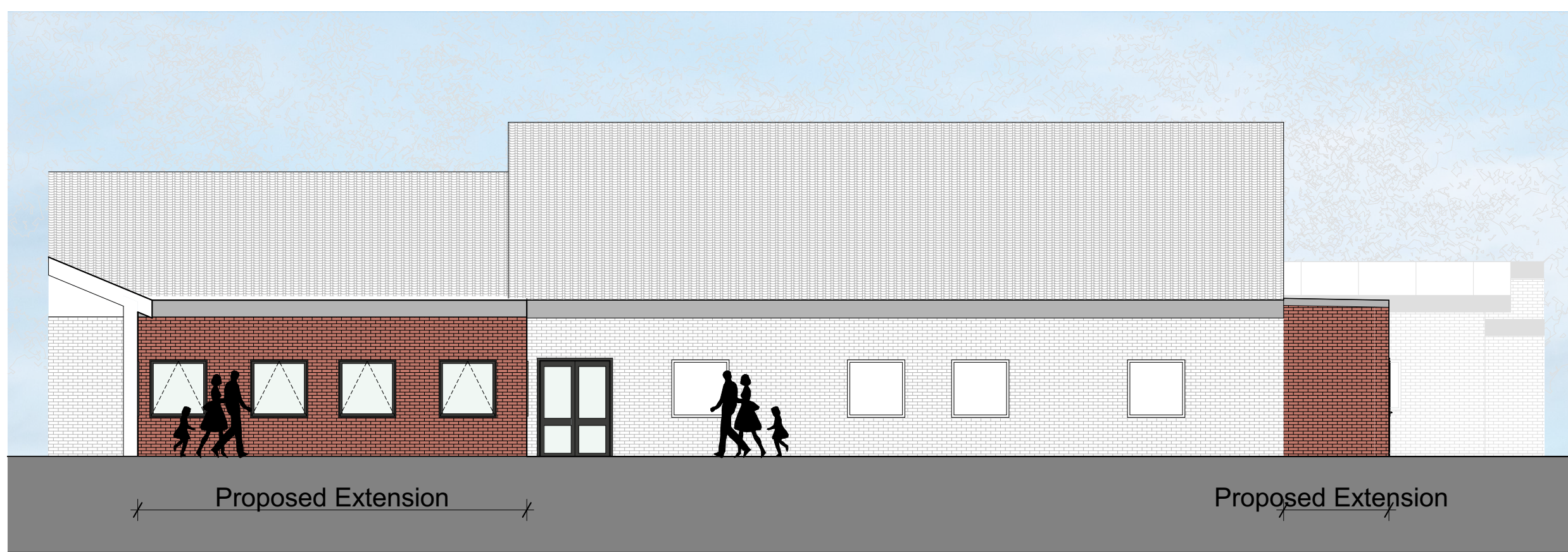
North Elevation Main School Building
