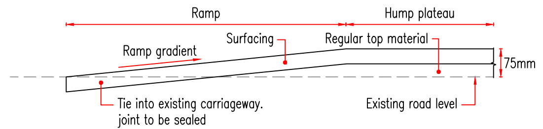
CONSTRUCTION DETAIL
