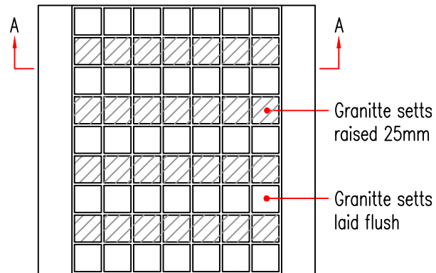
PLAN DETAIL
