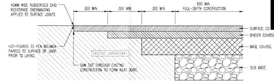
TYPICAL CARRIAGEWAY TIE-IN TO EXISTING CARRIAGEWAY DETAIL SCALE 1:10
