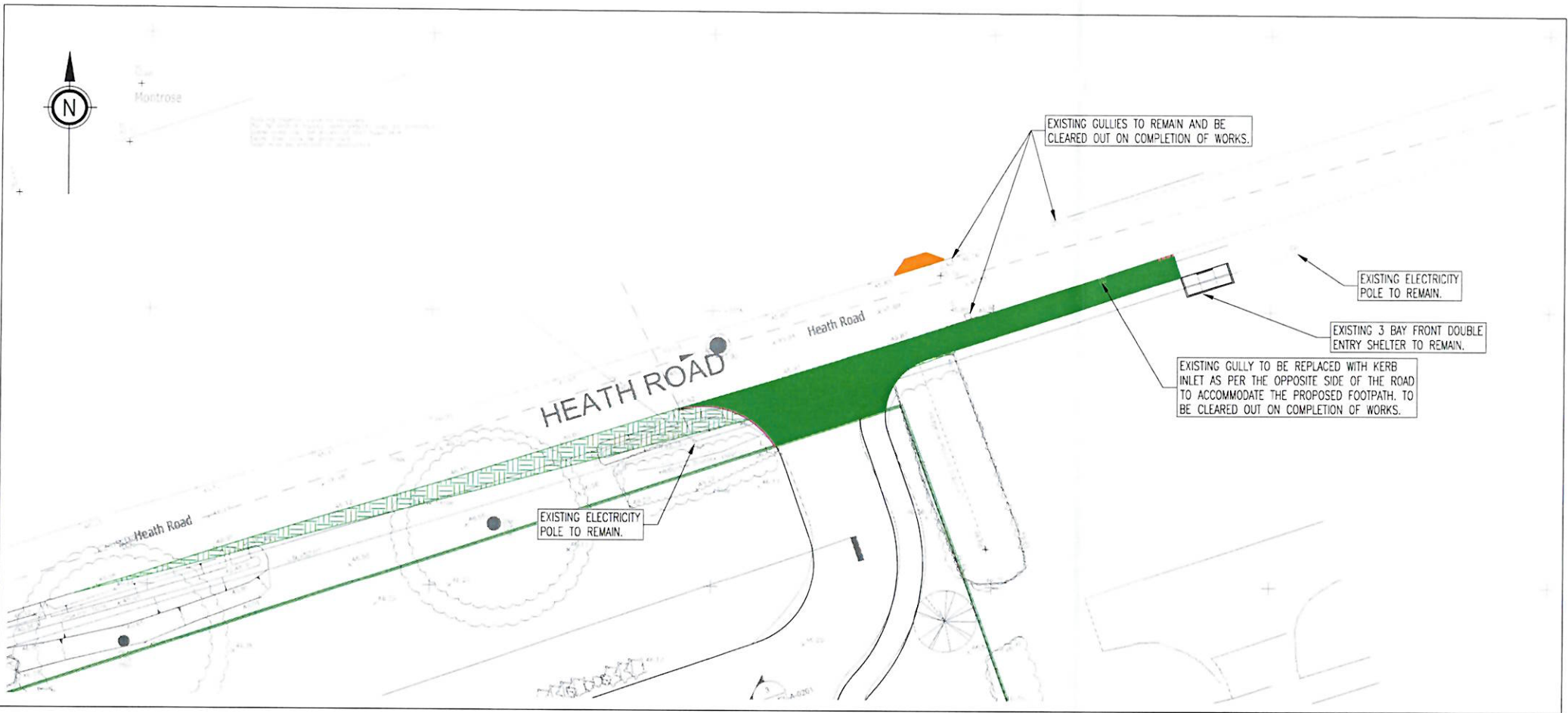
S278 SITE CLEARANCE
