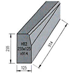
DROPPER KERB (DL1) LEFT SCALE 1:10
