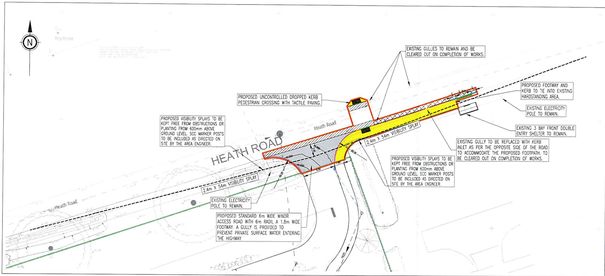
S278 GENERAL ARRANGEMENT
