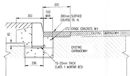
TYPICAL CARRIAGEWAY TIE-IN TO EXISTING CARRIAGEWAY DETAIL SCALE 1:10
