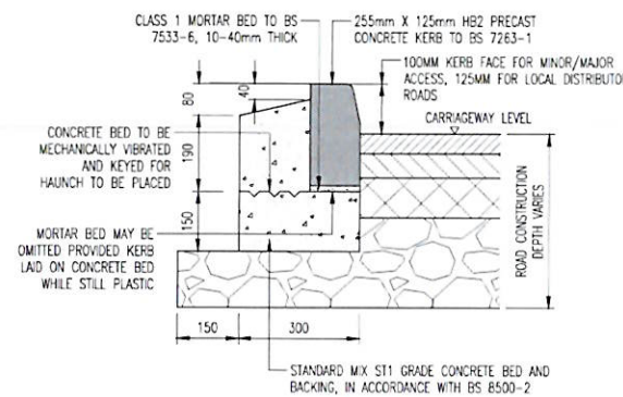
HALF-BATTERED KERB (HB2) DETAIL SCALE 1:10
