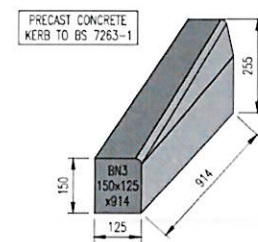
DROPPER KERB (DR1) RIGHT SCALE 1:10
