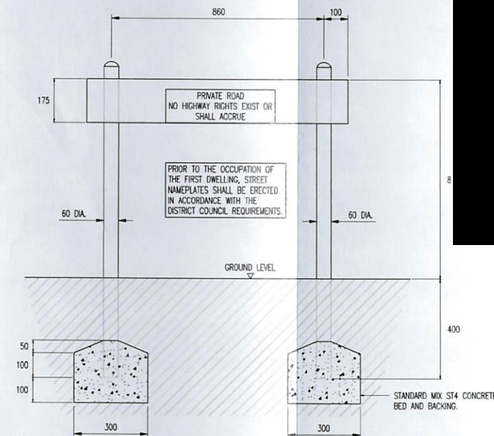
STREET NAME PLATE DETAIL
