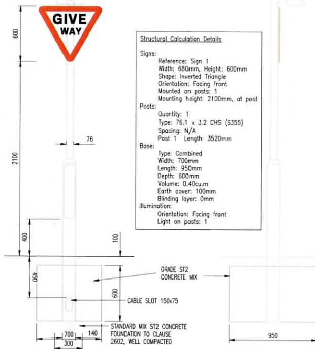
DIAGRAM 602 GIVE WAY SIGN (LIT) CONSTRUCTED IN FOOTWAY
