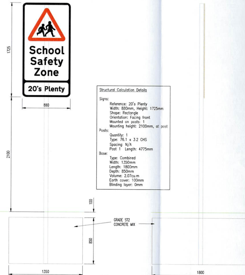
DIAGRAM 545 CHILDREN GOING TO OR FROM SCHOOL SIGN - CONSTRUCTED IN FOOTWAY
