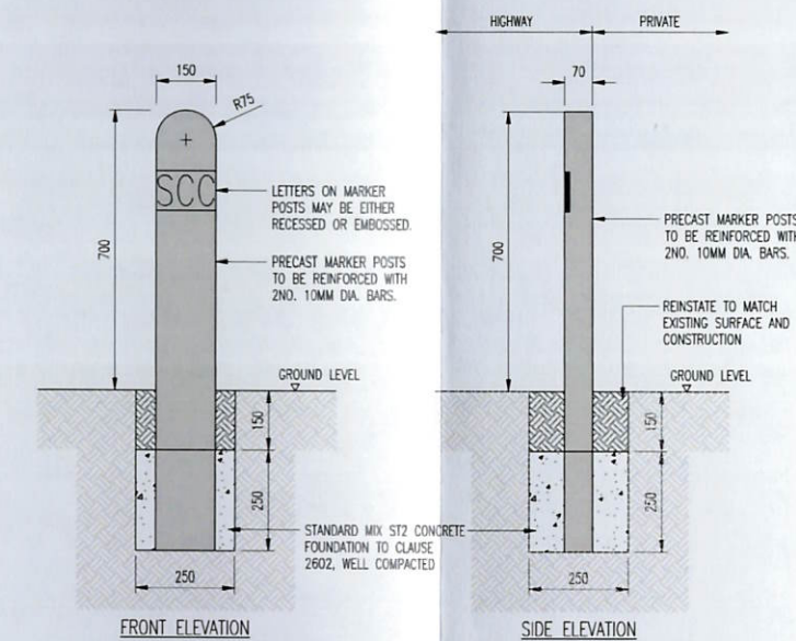
PRECAST CONCRETE BOUNDARY MARKER POST
