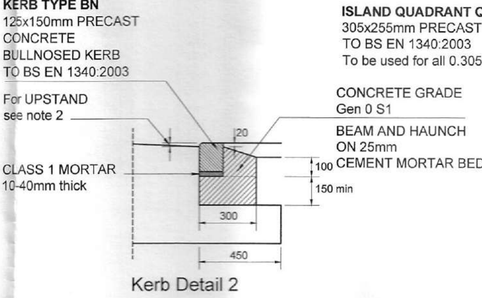
Kerb Detail 2
