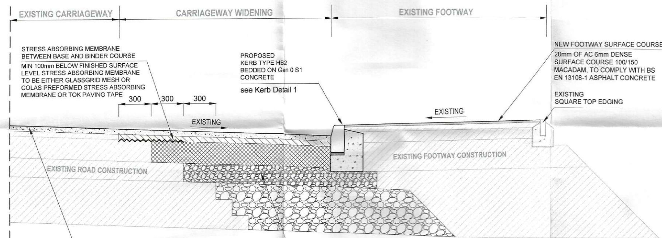
Typical section through existing tarmac road with proposed pedestrian crossing and refuge island detail
