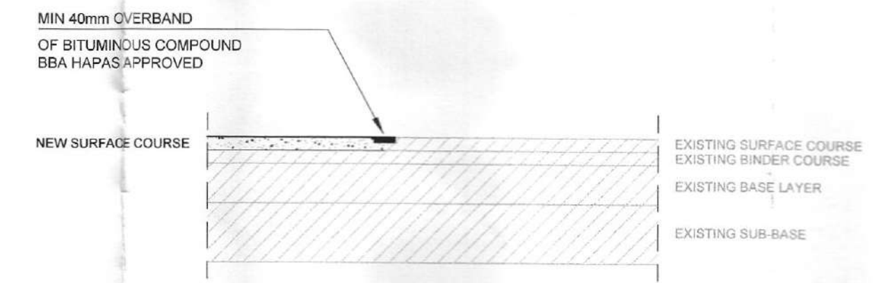
Surface Course Joining Detail
