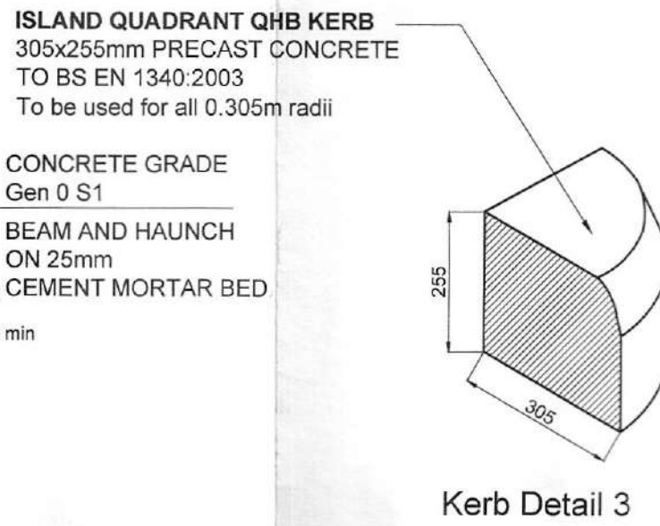
Kerb Detail 3
