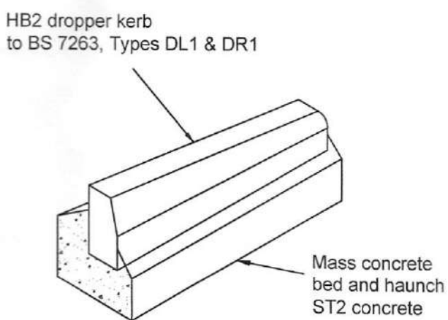
Dropper Transition Kerb Type DL1 (& DR1)
