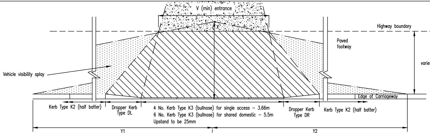
LAYOUT DM02
