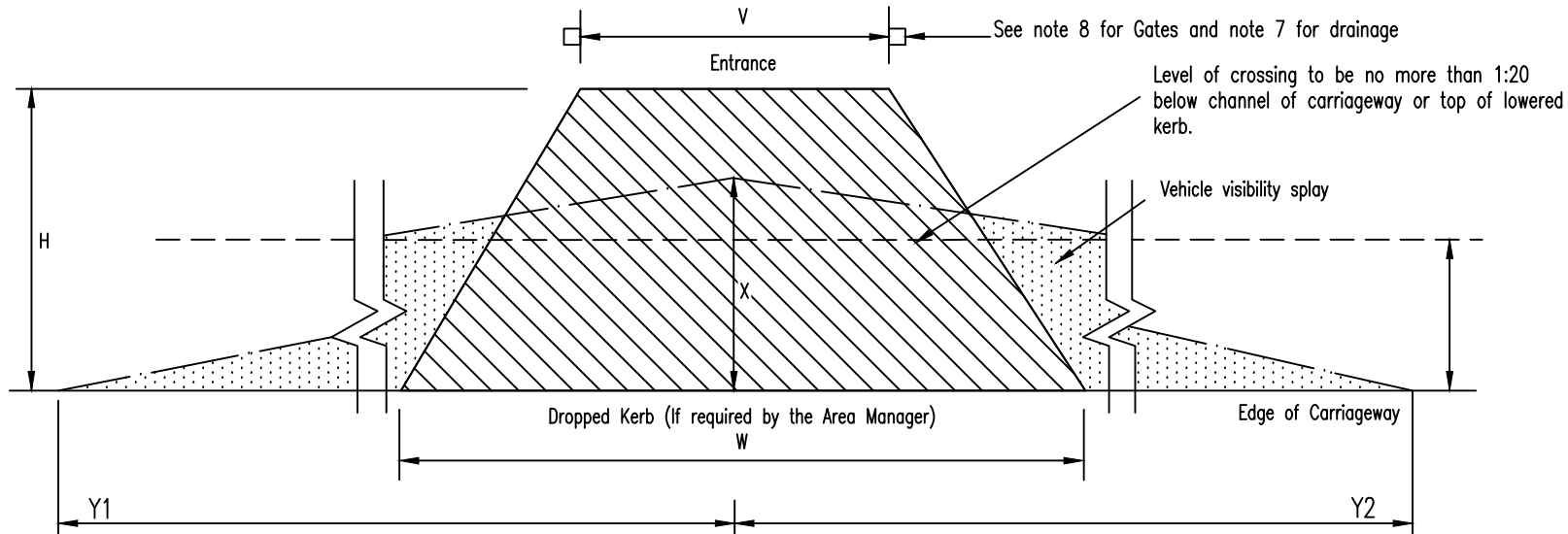
LAYOUT DM01
