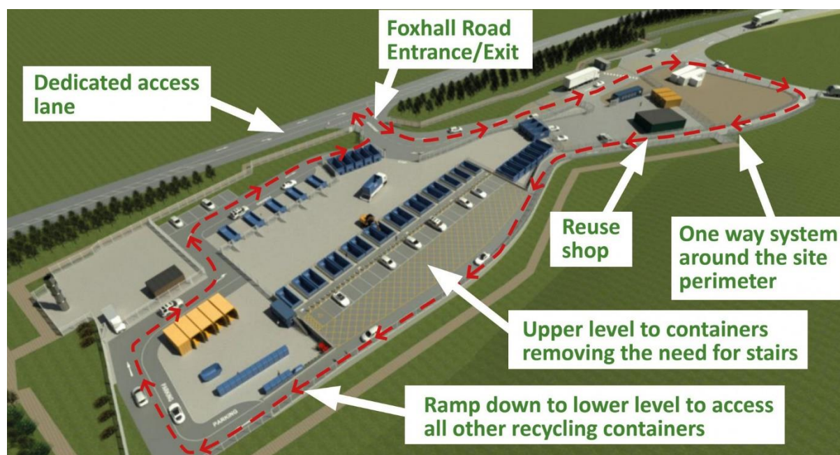
Proposed site layout for improvements of the Foxhall Household Waste & Recycling Centre, East Suffolk
